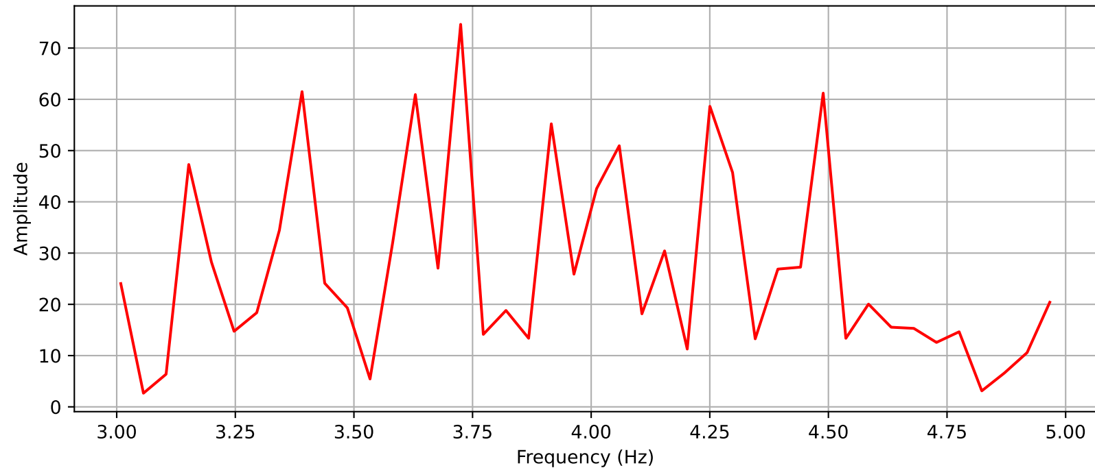
FIGURE 3 : Frequency spectrum - Task 1
